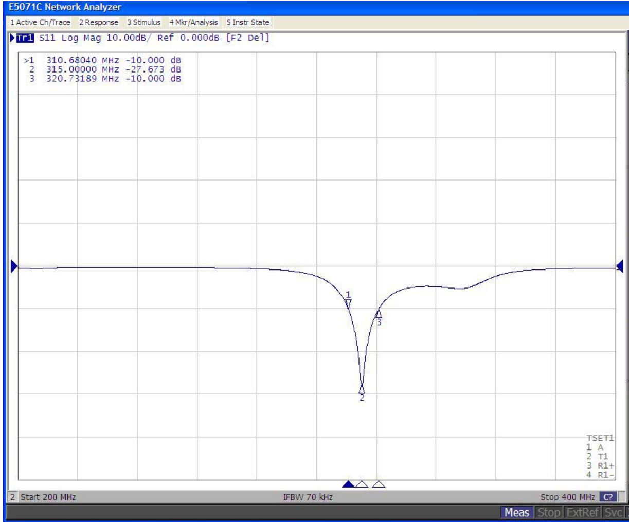
Fig. 4 Return loss
